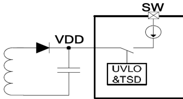
Fig 1. Startup circuit
