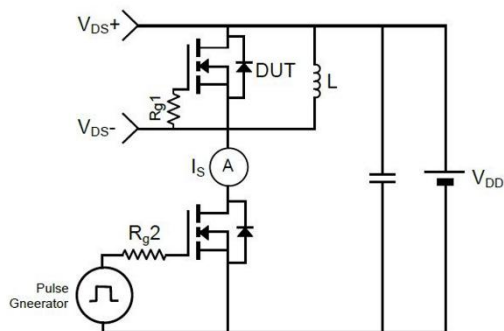
Fig 16. Diode Reverse Recovery Test Circuit & Waveforms
