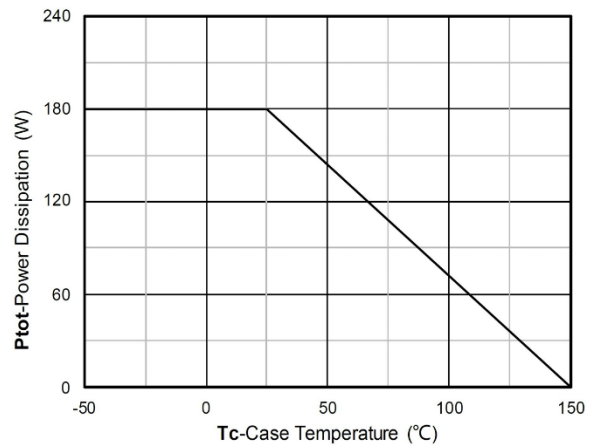
Fig 6. Typical Power Dissipation
