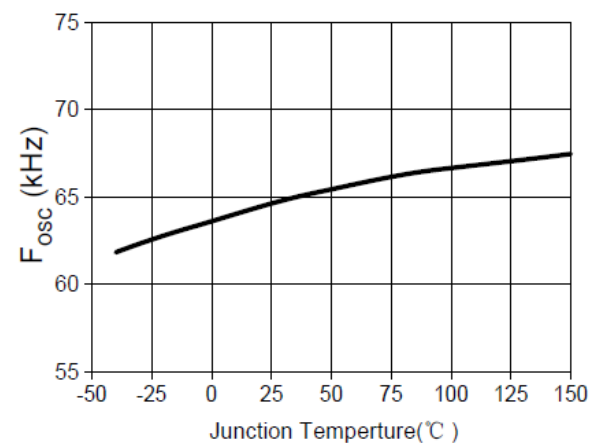
6. F_{osc} vs. T_J
