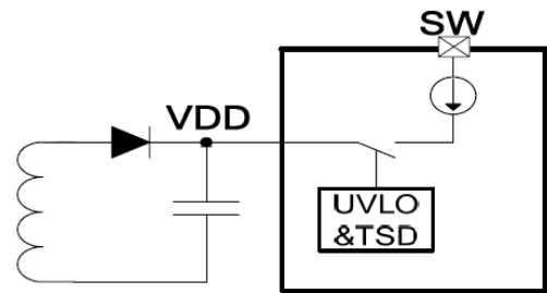
Fig 1. Startup circuit
