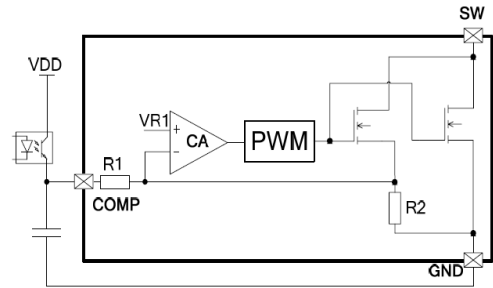
Fig 2. Feedback circuit
