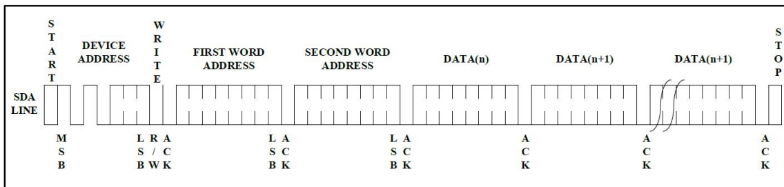
Figure 6 Page Write
