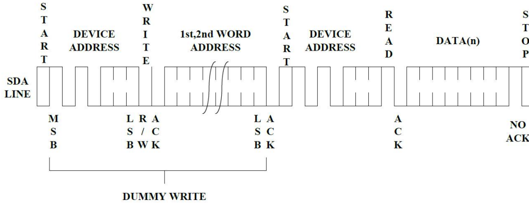
Figure 8 Random Read
