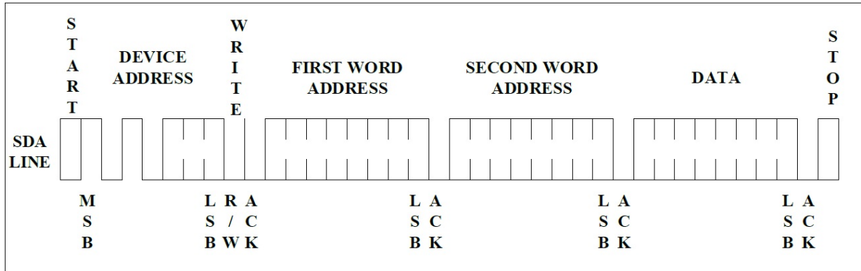
Figure 5 Byte Write
